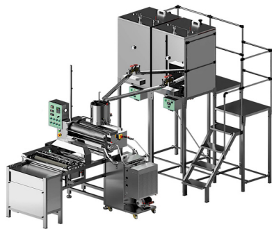
Full Automatic Beeswax Foundation Machine
